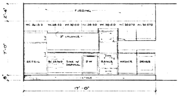
AUDITORIUM KITCHEN SCALE 1/4" = 1'-0"
