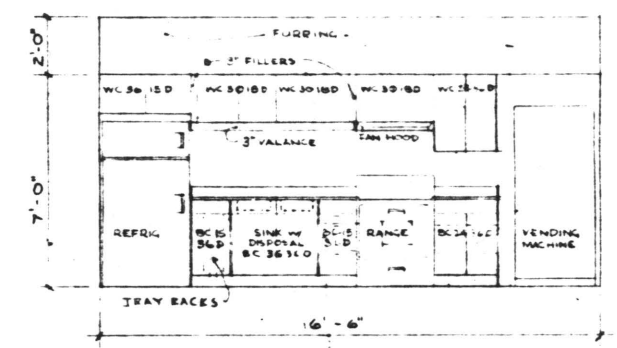
PREPARATION KITCHEN SCALE 1/4" = 1'-0"
