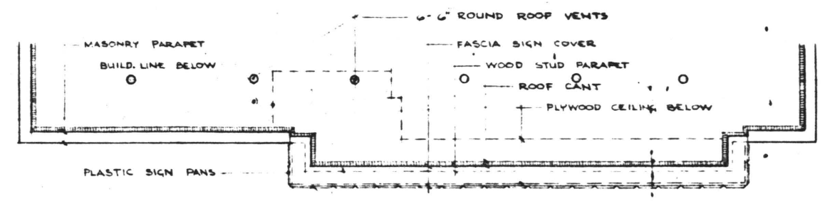
PARTIAL ROOF PLAN SCALE 1/8" = 1'-0"
